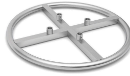
TOT-CIRCLE SKU: H10834 50 mm tube circle - Diameter 96 cm for Totem pole
