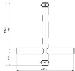
UNO-TW SKU: H11437 Suspension T for hanging a projector For 50 mm tube Manufactured to ISO DIN 4113 and TÜV standards White finish
